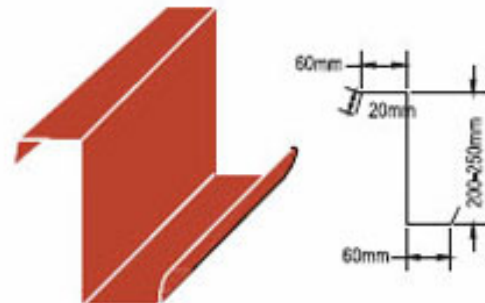
TYPICAL Z- SECTION
